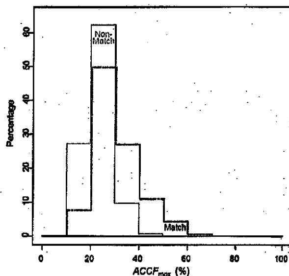
Figure 9-11. De Kinder breach face correlations: The green dashed lines depict a histogram of the matching scores, while the brown solid lines depict a histogram of the non-matching scores.
