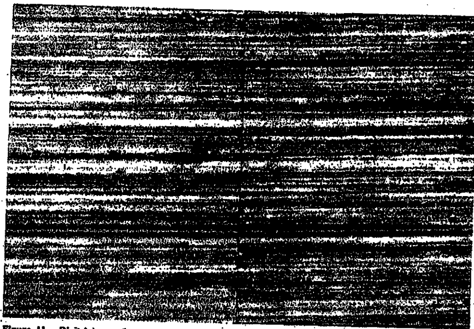
Figure 11. Digital image from comparison microscope of two consecutively made-in-house ground samples illustrating "coincident" matching striated areas.
