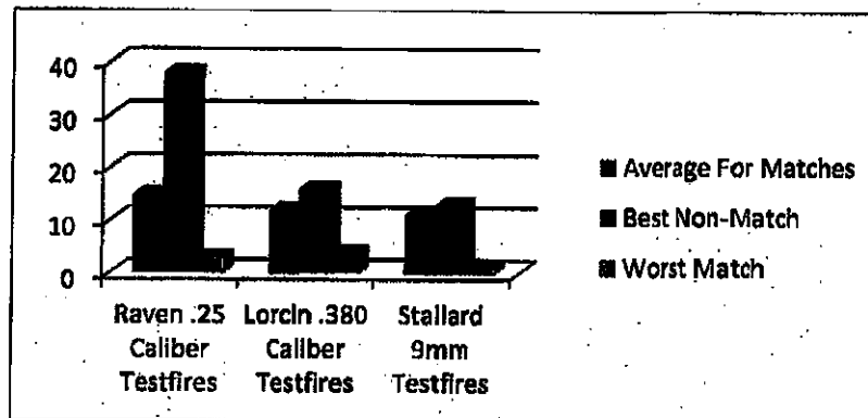
Percentage of Matching Two-Dimensional Striations in Single Land Impressions
